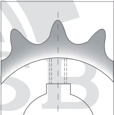
Teeth: Inductioned hardness HRC40-50 Finished bore tolerance HT. Roughness value RA1.6. Keyway to USAS B 17.1 1967
